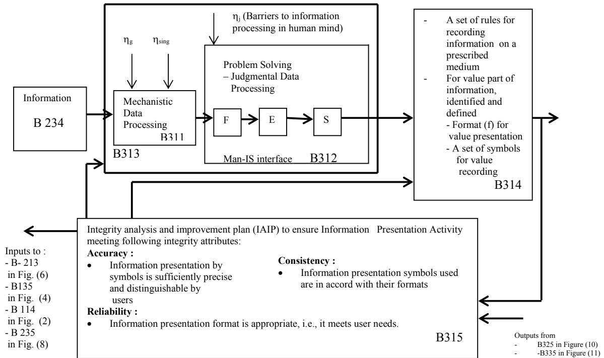
Figure 9 : Information Flow Model for Information Presentation Activity under Output Stage of Basic IS Model along with accompanying integrity analysis implications
